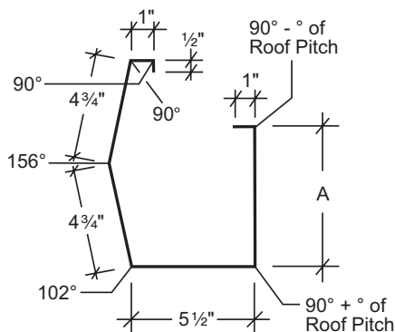
Sculptured Gutter
