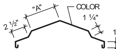
Ridge Flashing - For Ridge Vent
