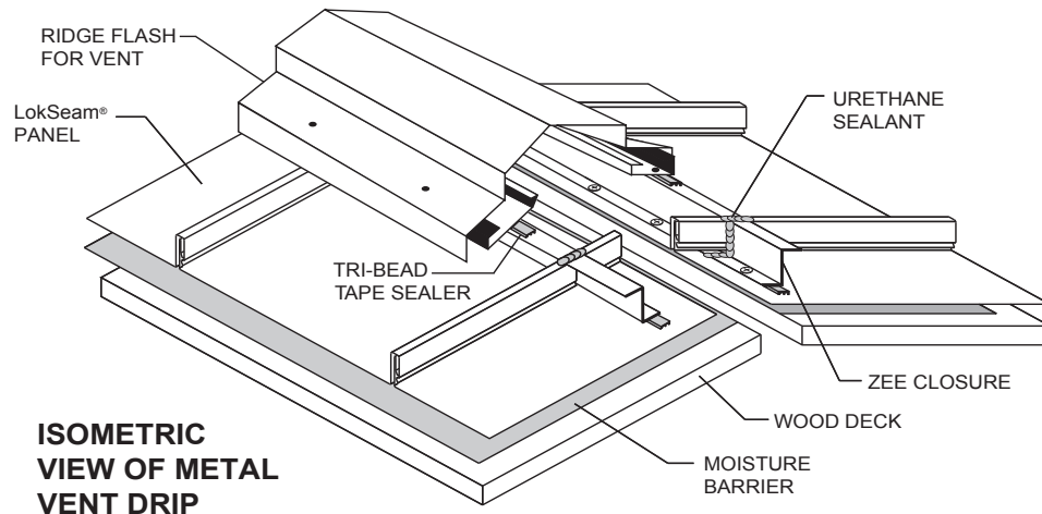
STANDARD RIDGE WITH PERFORATED VENT DRIP
