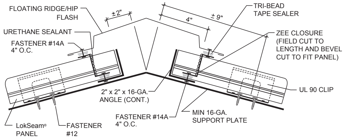
CROSS SECTION OF FLOATING HIP
