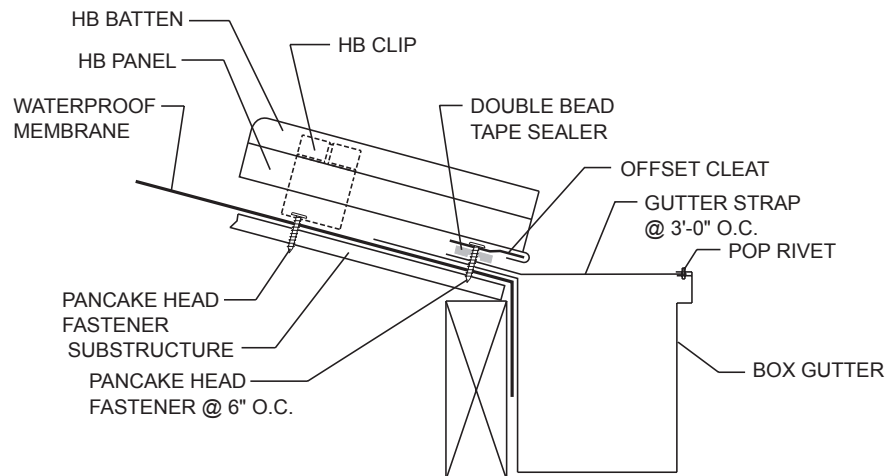
PANEL END DETAIL
