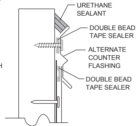
ALTERNATE DETAIL
