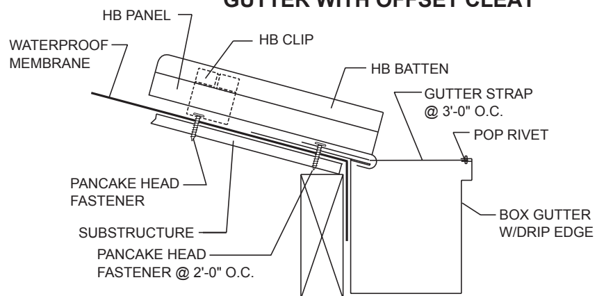
PANEL END DETAIL
