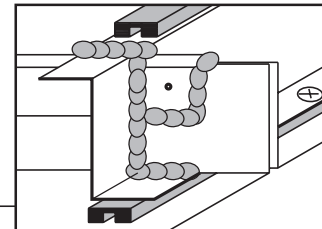
SEALANT DETAIL
