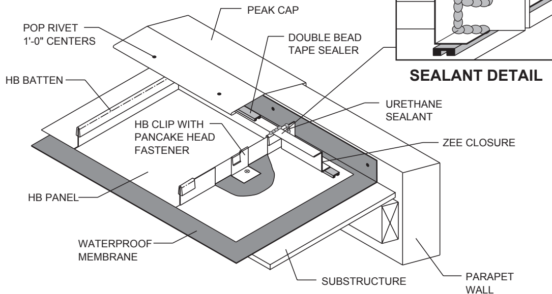
ISOMETRIC VIEW OF PEAK CAP
