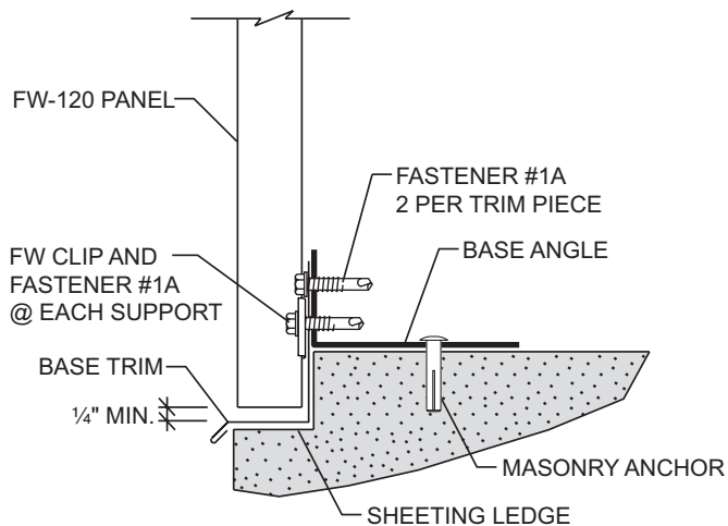
ALTERNATE DETAIL WITH SHEETING NOTCH
