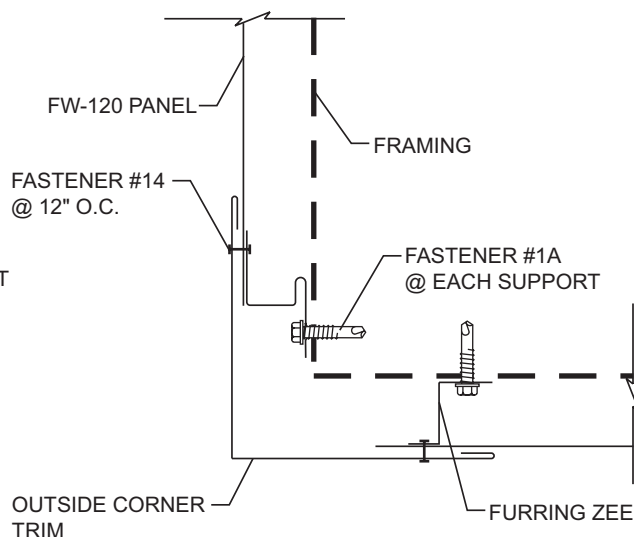
OUTSIDE CORNER
