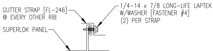
GUTTER STRAP ATTACHMENT
