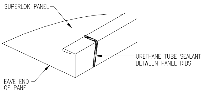
EAVE SEALANT DETAIL
