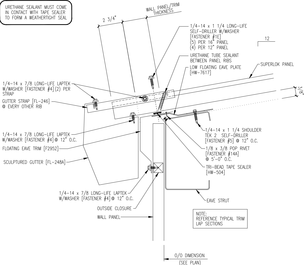
EAVE SEALANT DETAIL
