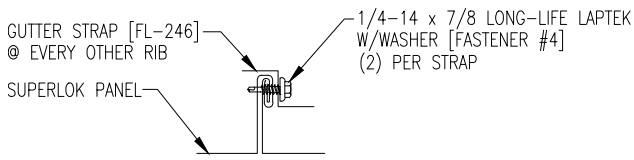
GUTTER STRAP ATTACHMENT
