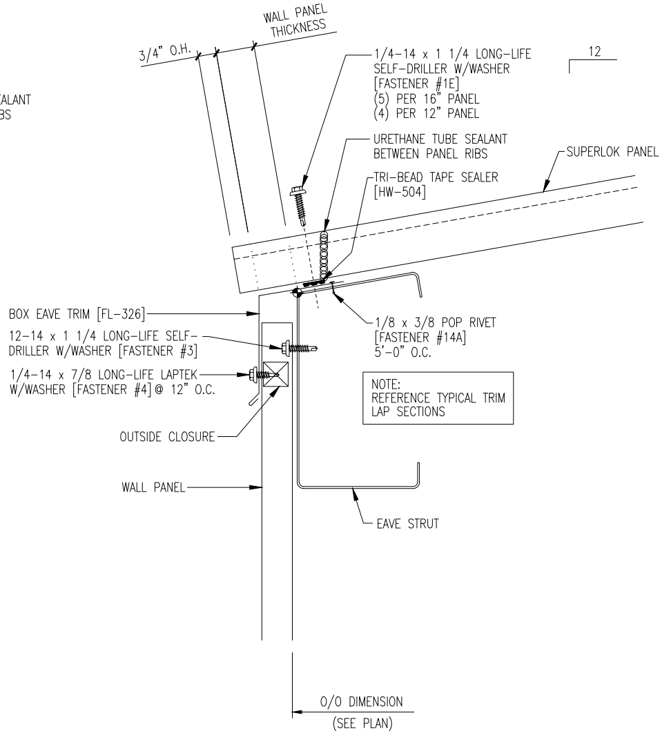
FASTENER SPACING @ EAVE
