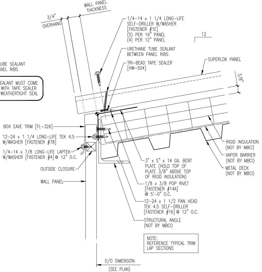
FASTENER SPACING @ EAVE
