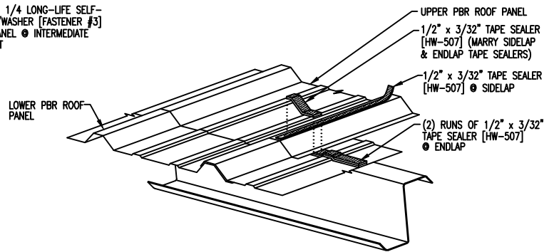
ENDLAP SEALANT DETAIL
