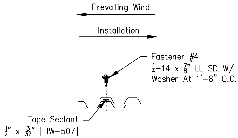
PBD Panel Sidelap
