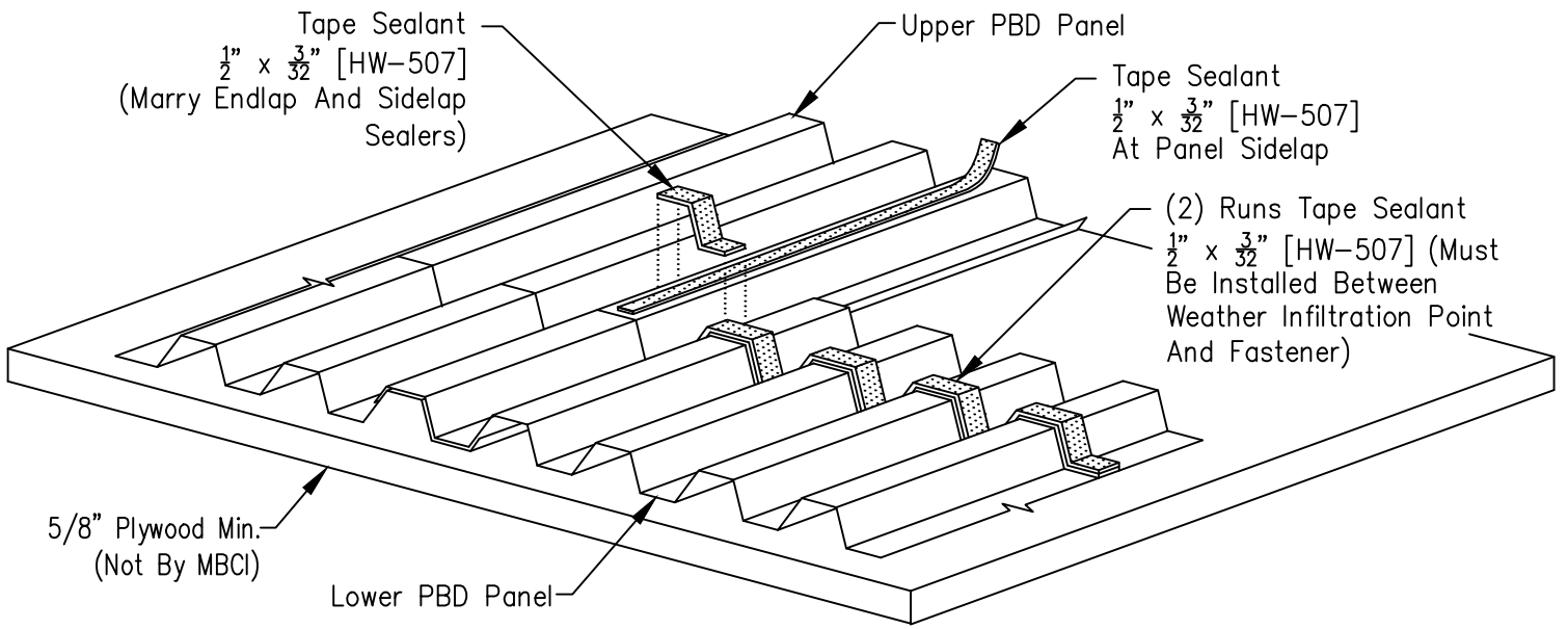
Endlap Sealant Detail
