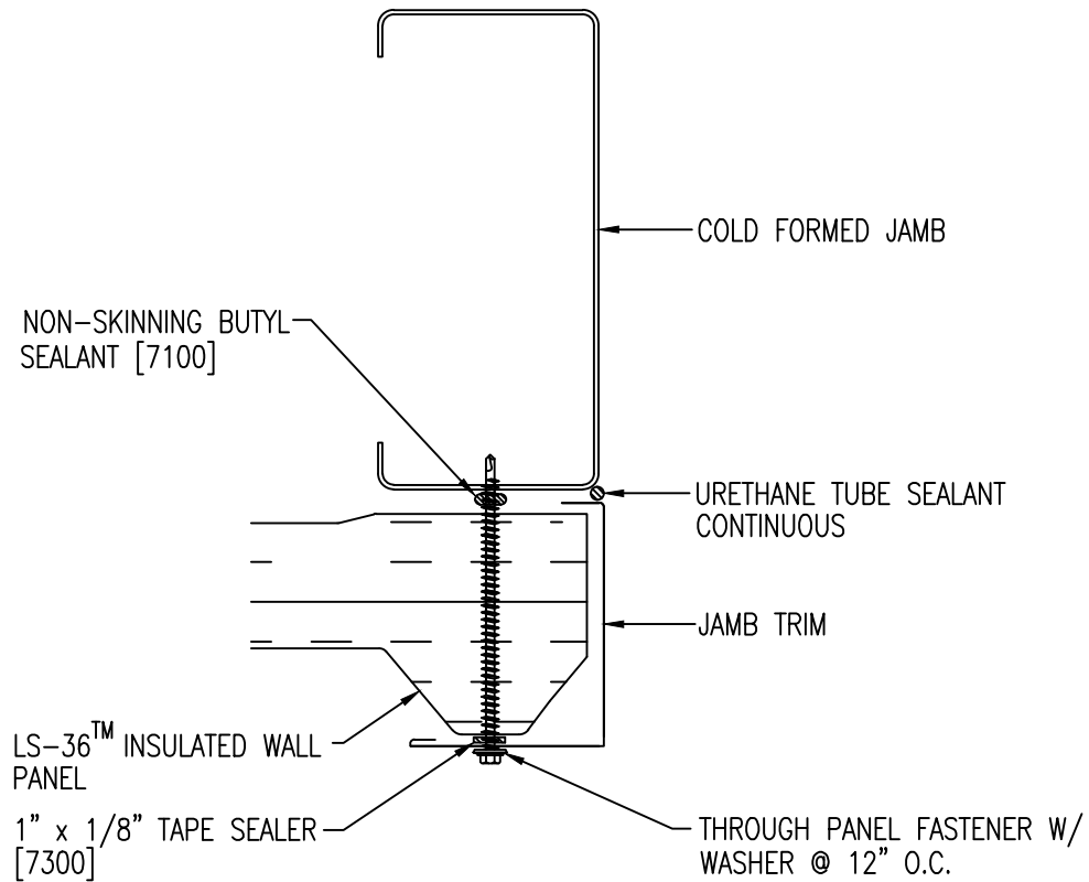
JAMB TRIM AT HIGH RIB
