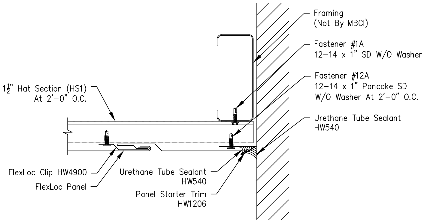
Panel Termination
