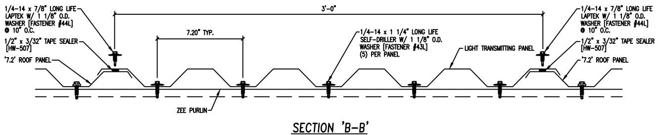
LIGHT TRANSMITTING PANEL INSTALLATION
