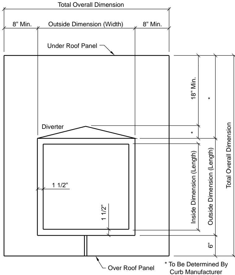
Plan View
