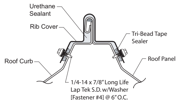
Rib Cover Attachment
