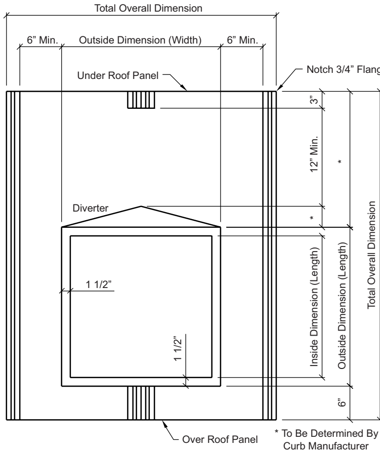
Plan View
