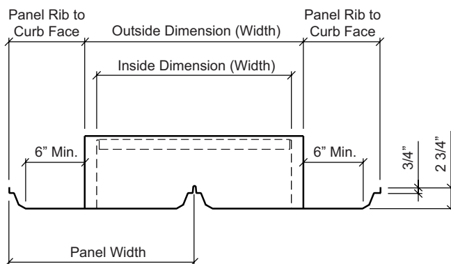
End View
