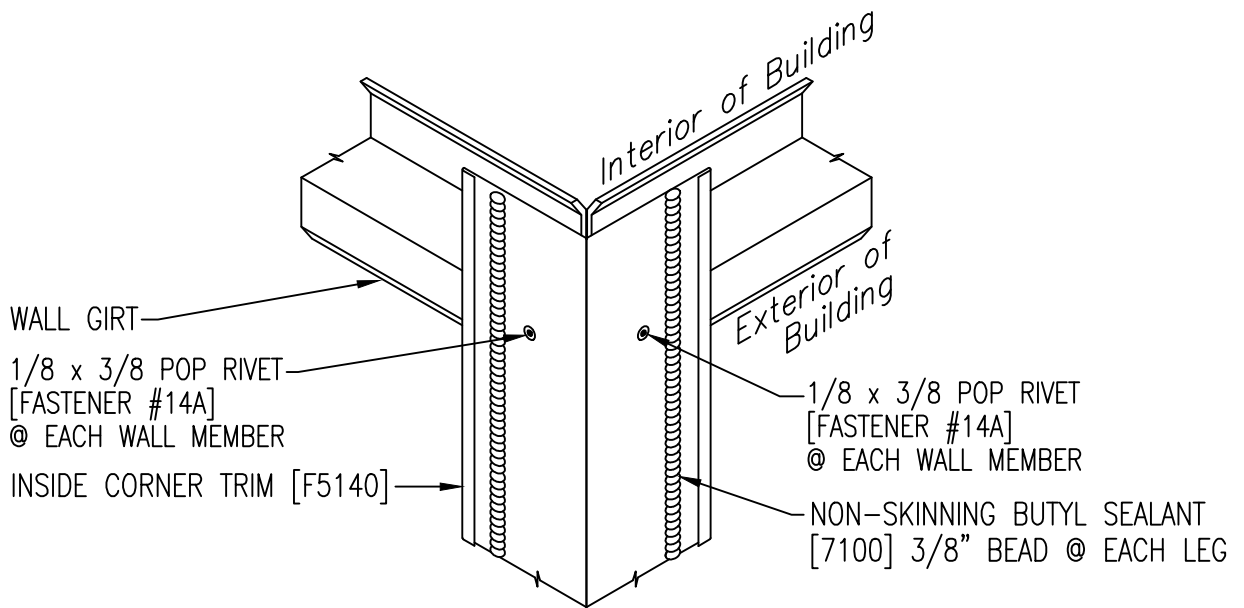
CORNER FRAMING & SEALANT AT INSIDE CORNER TRIM
