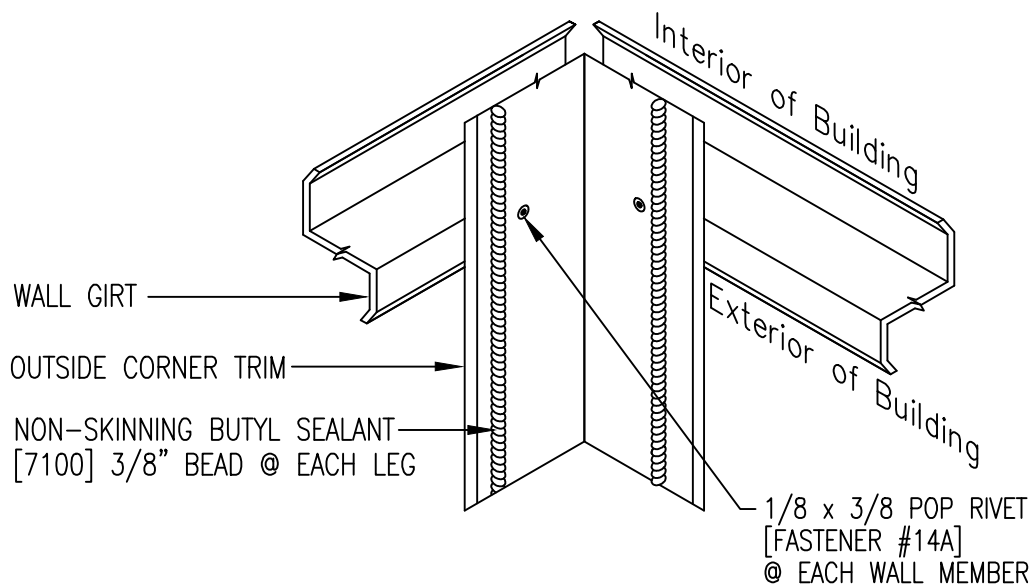
CORNER FRAMING & SEALANT AT INSIDE CORNER TRIM
