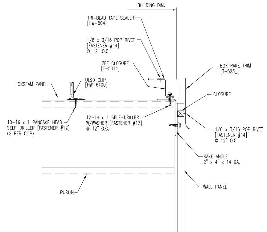
OFF - MODULE FIELD CUT AND BEND UP PANEL.
